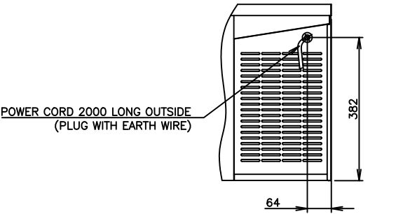
VIEW A (1/10)
