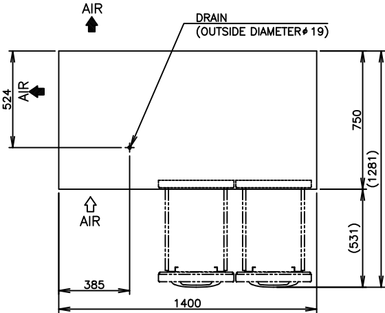
VIEW A (1/10)
